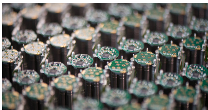
Precision milling – milling of singulated boards with a xy mechanical precision below 50 micrometers
